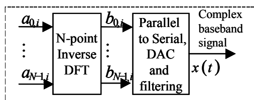
Fig. 1. An OFDM transmitter
