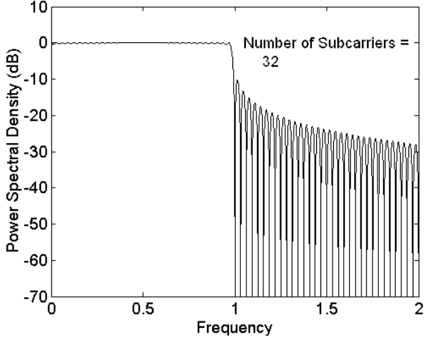
Fig. 3(a). Power spectrum of an OFDM signal with 32 subcarriers
