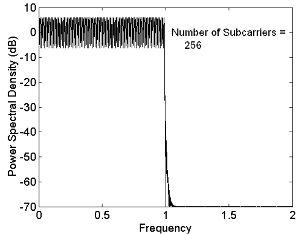
Fig. 5(d) Modulation in groups of three, 256 subcarriers
