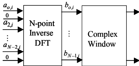
Fig. 7. Time domain equivalent to weighting pairs of subcarriers
