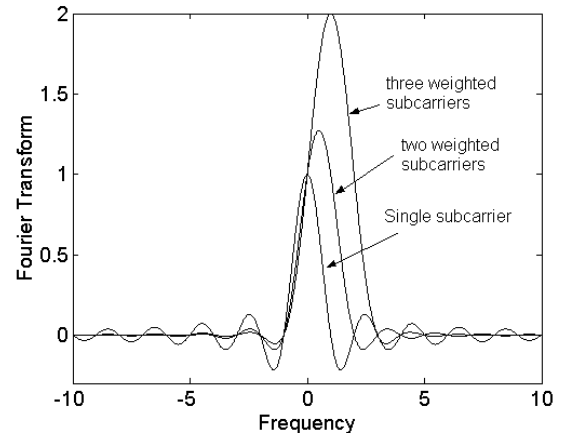
Fig. 4. Fourier transforms of weighted groups of subcarriers
