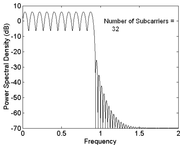
Fig. 5 (c) Modulation in groups of three, 32 subcarriers
