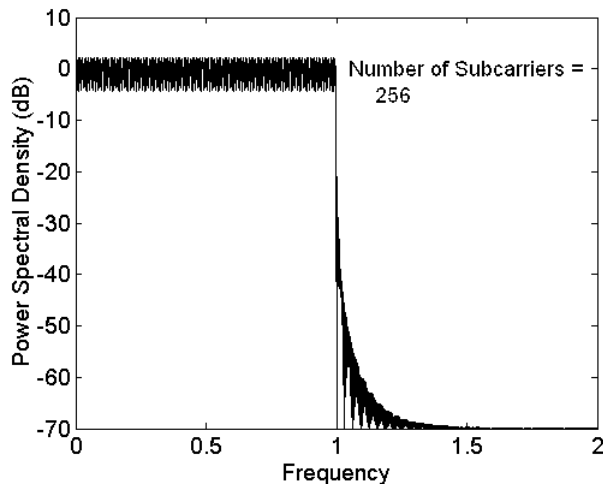
Fig. 5 (b) Modulation in pairs, 256 subcarriers
