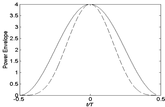
Fig. 6. Variation in the power envelope across a symbol period for PCC OFDM. Solid line m = 2 , dotted line m = 3 .
