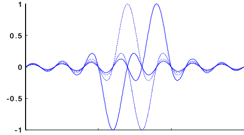
Fig. 2. Fourier Transforms of four adjacent OFDM subcarriers.
