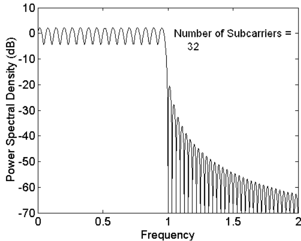
Fig. 5(a). Modulation in pairs, 32 subcarriers
