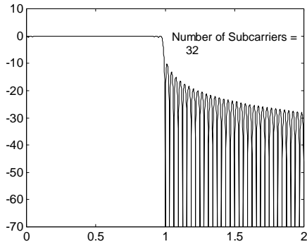
Figure 3(a). Power spectrum of an OFDM signal with 32 subcarriers
