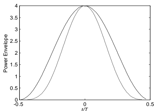
Figure 6. Variation in the power envelope across a symbol period for PCC OFDM. Solid line m = 2 , dotted line m = 3 .
