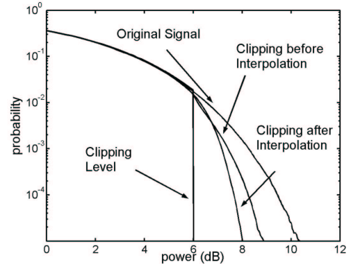
Figure 2. Complementary cumulative distribution of signal amplitude for HIPERLAN2
